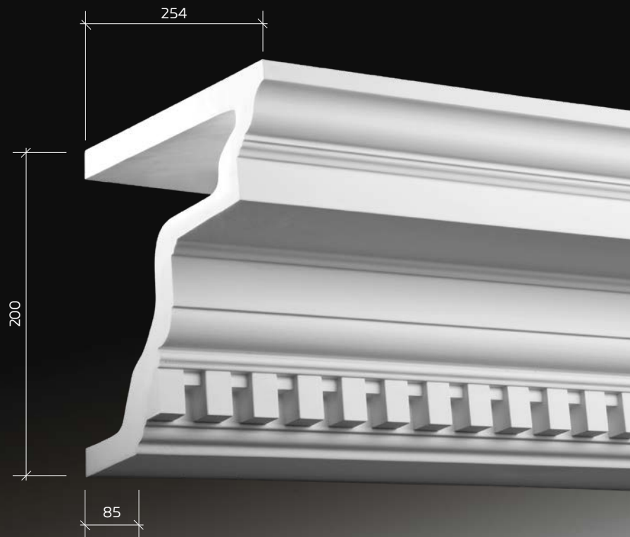
4.31.302 карниз
